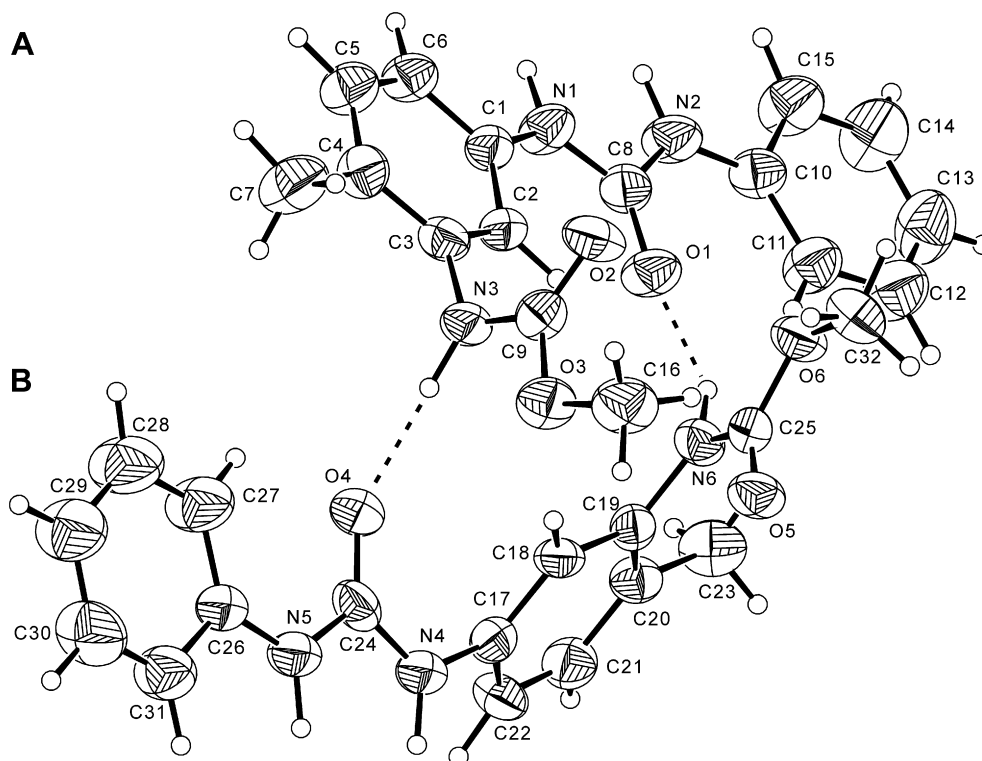
Fig. 2. Molecular structure of 1 . Two unsymmetrical units are depicted. A complementary hydrogen bond is indicated by the dotted line.
