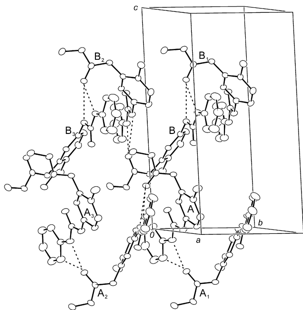
Fig. 3. Hydrogen-bond network of 1 . The hydrogen bonds are indicated by the dotted line. The molecules are given by the following symmetry operation; A_1 : -x, y + 0.5, -z , A_2 : -x, y - 0.5, -z , A_3 : x, y - 1, z , B_1 : -x, y + 0.5, -z + 1 , B_2 : -x, y - 0.5, -z + 1 , B_3 : x, y - 1, z .
