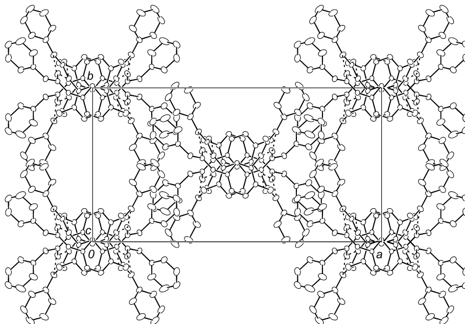
Fig. 5. Hydrogen-bond network of 2 . The disordered benzene molecules are omitted for clarity. The hydrogen bonds are indicated by the dotted line.
