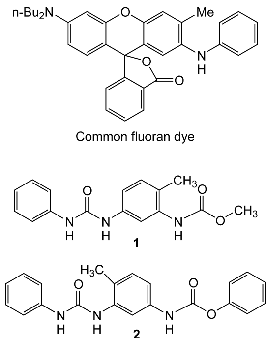
Fig. 1. Chemical structure of a common fluoran dye and UU derivatives.
