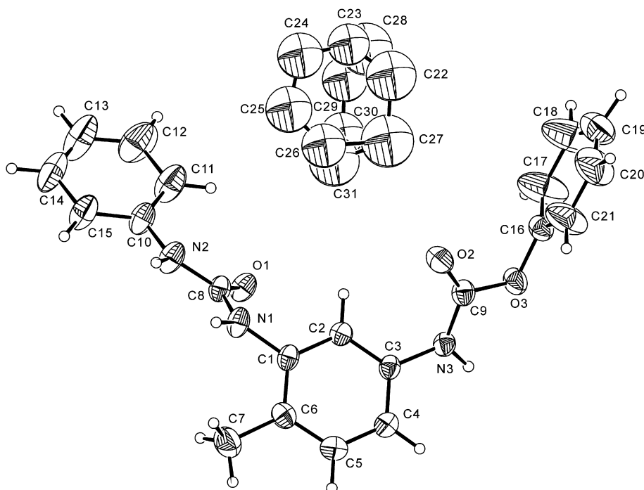
Fig. 4. Molecular structure of 2 with the disordered benzene.
